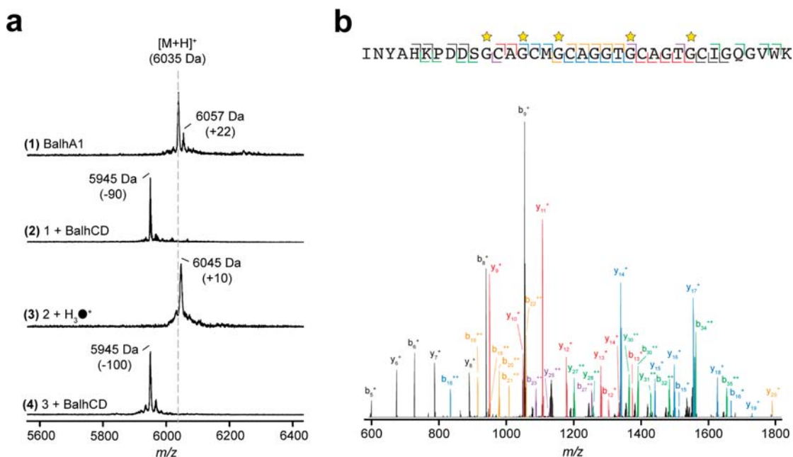
Figure 2. Site-specific incorporation of ^{18}O labels into BalhA1. (a) An overlay of MALDI-TOF MS spectra displaying the ^{18}O exchange process. Mass labels correspond to the 1+ charge state, and all mass shifts are reported relative to the pertinent noncyclized species (spectra 1 and 3). The loss of the ^{18}O labels in [ ^{18}O_5 ]-BalhA1 upon retreatment with BalhCD is evidenced by the loss of 100 Da (compared to -90 Da for BalhA1). ^{18}O labels are represented by filled circles. (b) The FT-MS/MS spectrum of trypsin-digested [ ^{18}O_5 ]-BalhA1. The b and y ions are colored based on the number of ^{18}O labels present in the fragment (green = 5; purple = 4; orange = 3; blue = 2; red = 1; black = 0). Stars represent the location of the ^{18}O labels.
