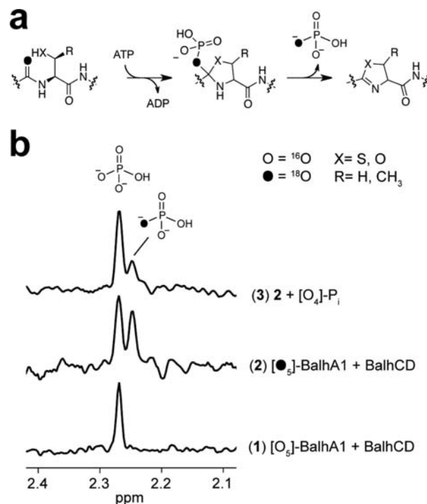
Figure 6. 31 P NMR of 18 O 5 -BalhA1 reactions. (a) The putative carbonyl oxygen phosphorylation mechanism for ATP utilization is displayed along with 31 P NMR spectra for both [ 18 O 5 ]-BalhA1 and [ 18 O 5 ]-BalhA1 reactions (b). The identity of the [ 16 O 4 ]-P i peak was verified by spiking the sample with a P i standard (spectrum 3).
