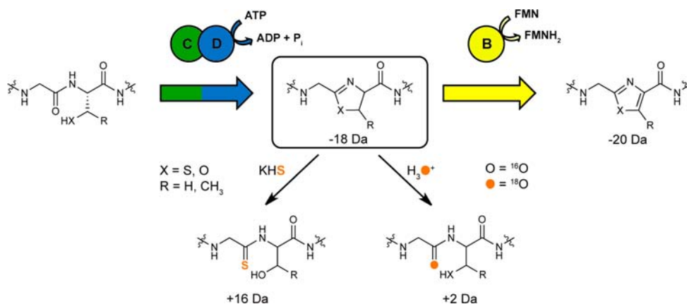
Figure 1. Azoline heterocycles are versatile intermediates for selective peptide labeling. A general scheme for TOMM heterocycle biogenesis is displayed. Select Cys, Ser, and Thr residues are cyclized by the ATP-dependent cyclodehydratase (complex of C and D proteins). Azoline heterocycles can then be oxidized by a flavin-dependent dehydrogenase to afford the aromatic azole. Alternatively, the electrophilic azoline heterocycle can be exploited for the installation of oxygen isotopes and thioamides using [ ^{18}O ]- H_2O and potassium hydrosulfide (KHS) as nucleophilic ring-opening agents, respectively. The mass shift relative to unmodified peptide is displayed underneath each product.
