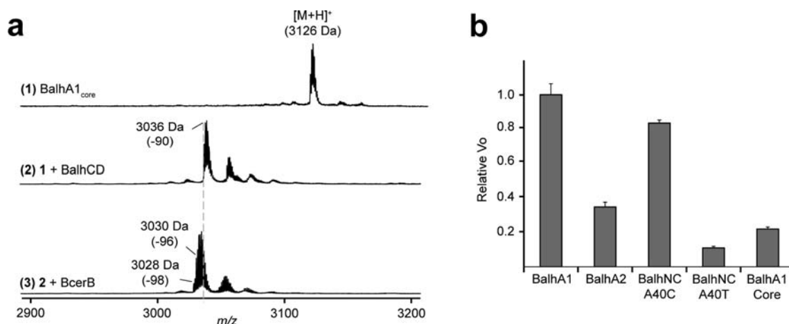
Figure 4. BalhA1 core processing. (a) An overlay of MALDI-TOF MS spectra displaying BalhCD- and BcerB/BalhCD-treated BalhA1 core . Mass labels correspond to the 1+ charge state, and all mass shifts are reported relative to the unmodified species (spectrum 1). (b) Relative processing rates for previously reported leader peptide-containing substrates of BalhCD are displayed alongside the processing rate for BalhA1 core . Error bars represent standard deviation from the mean ( n = 3 ).
